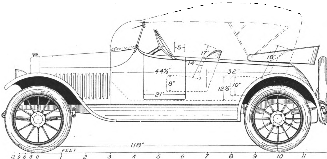
An Attractive Close-Coupled Four-Passenger Body Designed by George J. Mercer
